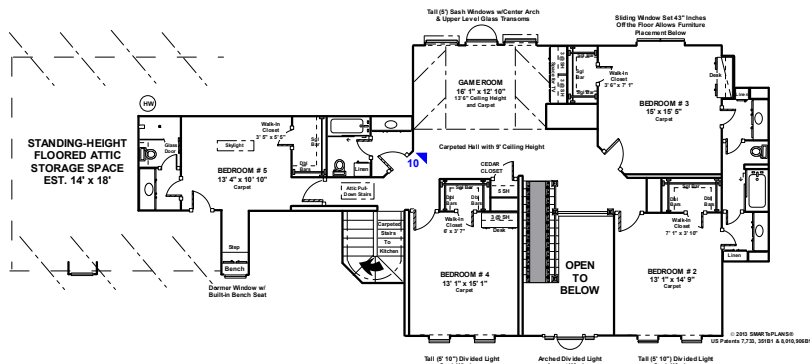
SECOND FLOOR
