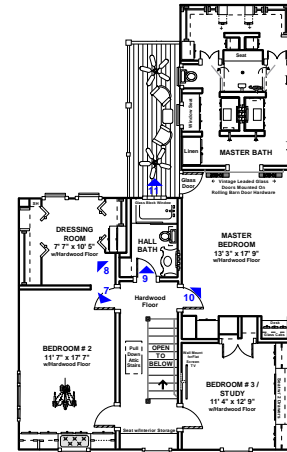
SECOND FLOOR
